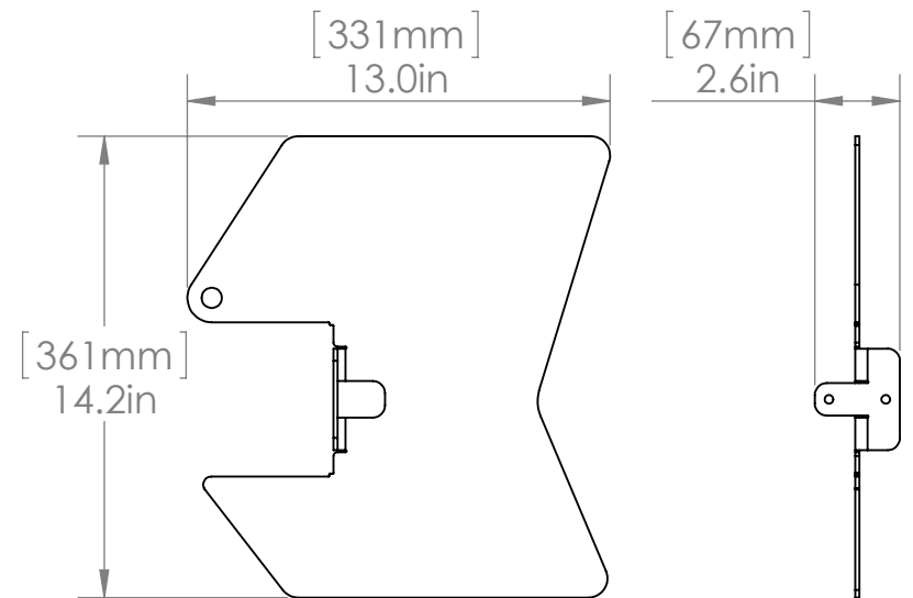
TAIL (1/TURBINE)
